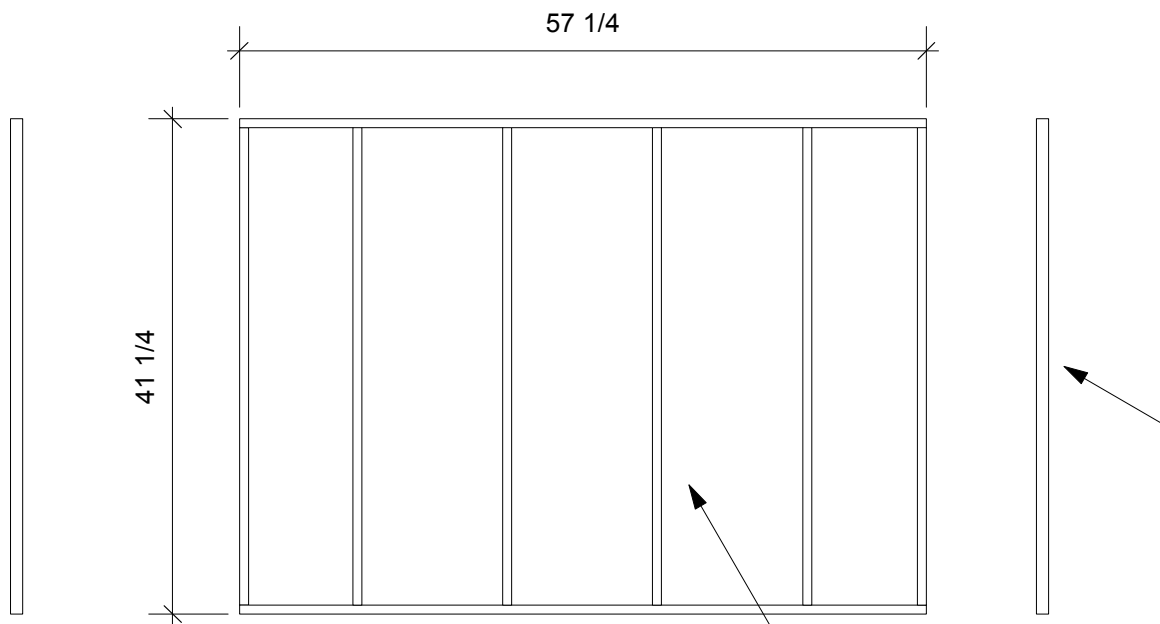
Front View Torsion wall made from 3/4" ply
