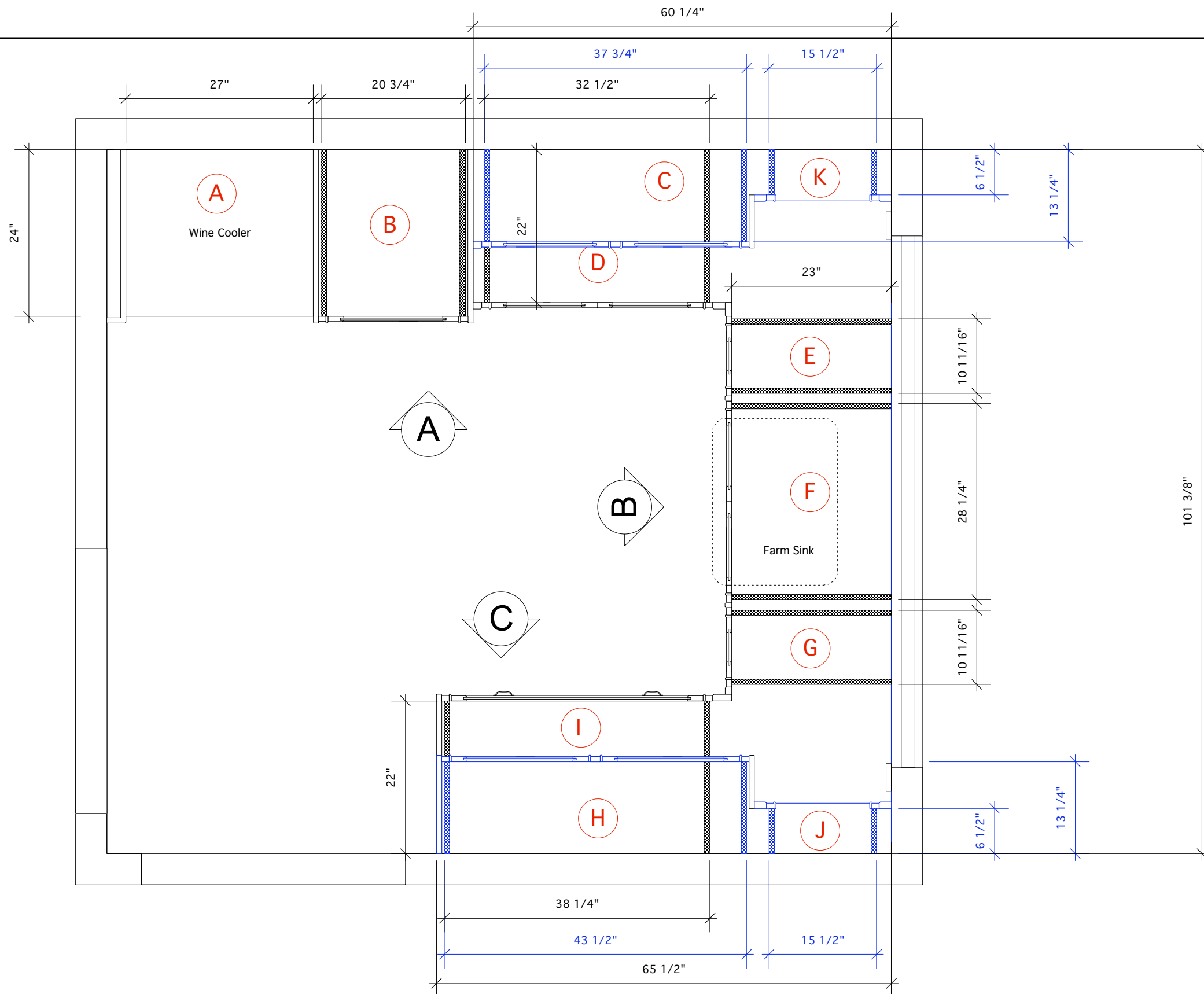
Room 14 - Pantry - Floorplan
